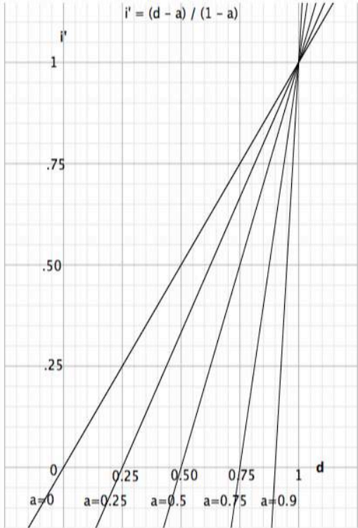
Figure 11. Inference from OR to IF-NOT. Variation of i' = P(C/NOT-A) as a function of d = P(A \text{ OR } C) for various values of a = P(A) .
